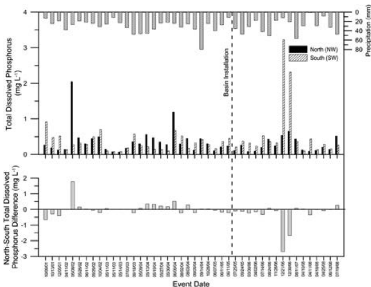
Fig. 4. Total runoff total dissolved phosphorus (TDP) minus base-flow total TDP per event ( \text{mg L}^{-1} ) and precipitation (mm) for each of the 44 sampled events from 2001 to 2008 at both north (NW) and south (SW) watersheds. Difference in total runoff total TDP minus base-flow total TDP (north–south) is also presented.
