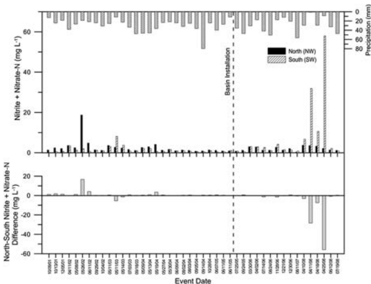
Fig. 6. Total runoff nitrite + nitrate-N ( \text{NO}_2+\text{NO}_3 ) minus base-flow \text{NO}_2+\text{NO}_3\text{-N} per event ( \text{mg L}^{-1} ) and precipitation (mm) for each of the 44 sampled events from 2001 to 2008 at both north (NW) and south (SW) watersheds. Difference in total runoff \text{NO}_2+\text{NO}_3\text{-N} minus base-flow \text{NO}_2+\text{NO}_3\text{-N} (north–south) is also presented.
