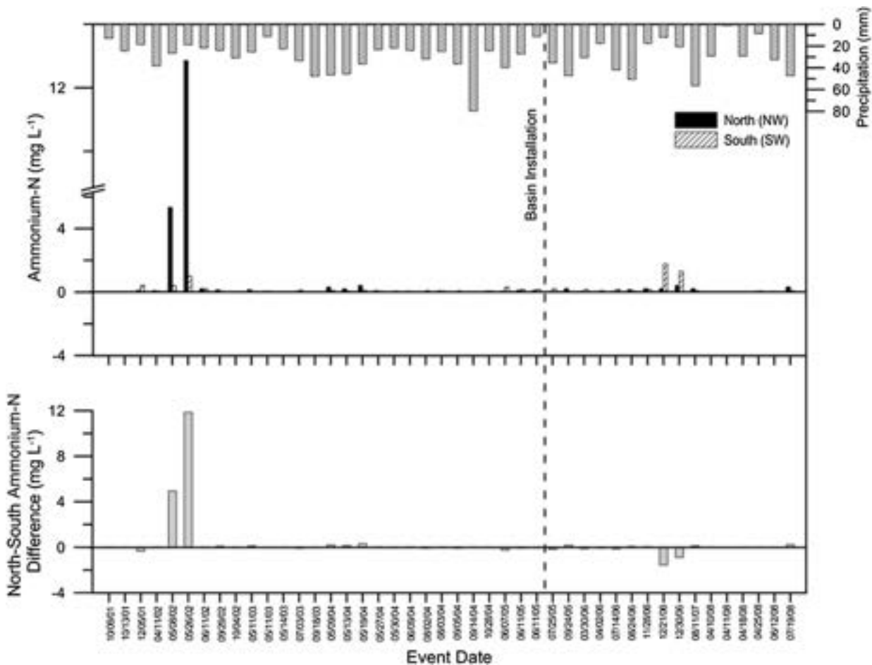
Fig. 7. Total runoff ammonium-N ( NH_4-N ) minus base-flow NH_4-N per event ( mg L^{-1} ) and precipitation (mm) for each of the 44 sampled events from 2001 to 2008 at both north (NW) and south (SW) watersheds. Difference in total runoff NH_4-N minus base-flow NH_4-N (north–south) is also presented.
