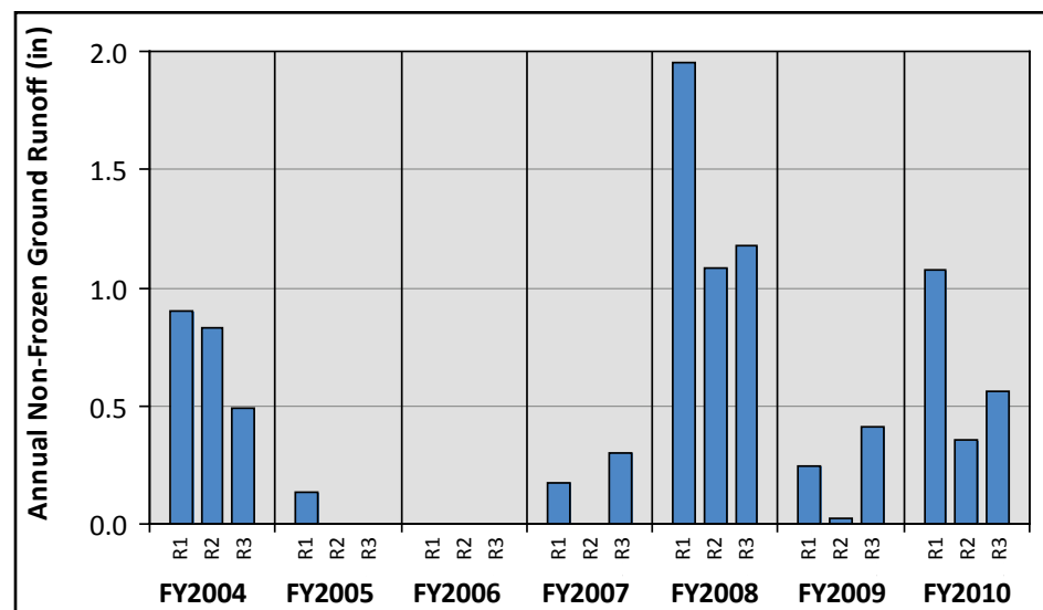
Figure 24. Annual non-frozen ground runoff
